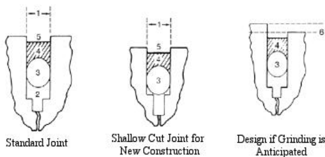
Figure 1: Good Joint Design
